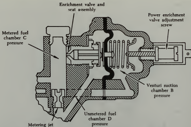
FIGURE 3-31. Airflow power enrichment valve.
